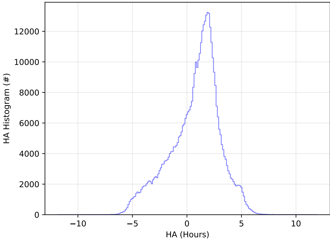
ddf_acor_sf10_lsf20_lsr50_v3.4_10yrs All sky z band: HA Histogram
