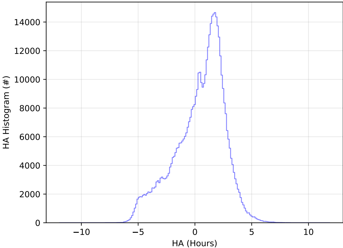
ddf_acor_sf10_lsf20_lsr50_v3.4_10yrs All sky r band: HA Histogram
