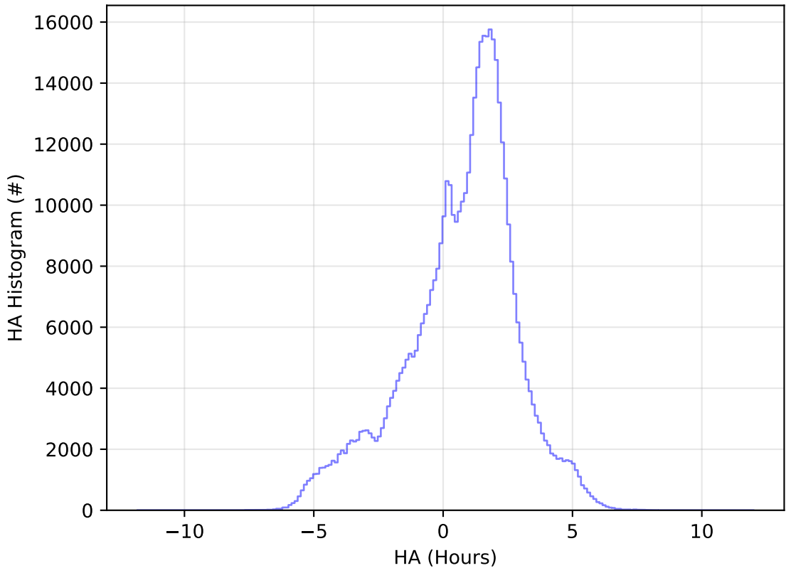
ddf_acor_sf10_lsf20_lsr50_v3.4_10yrs All sky i band: HA Histogram
