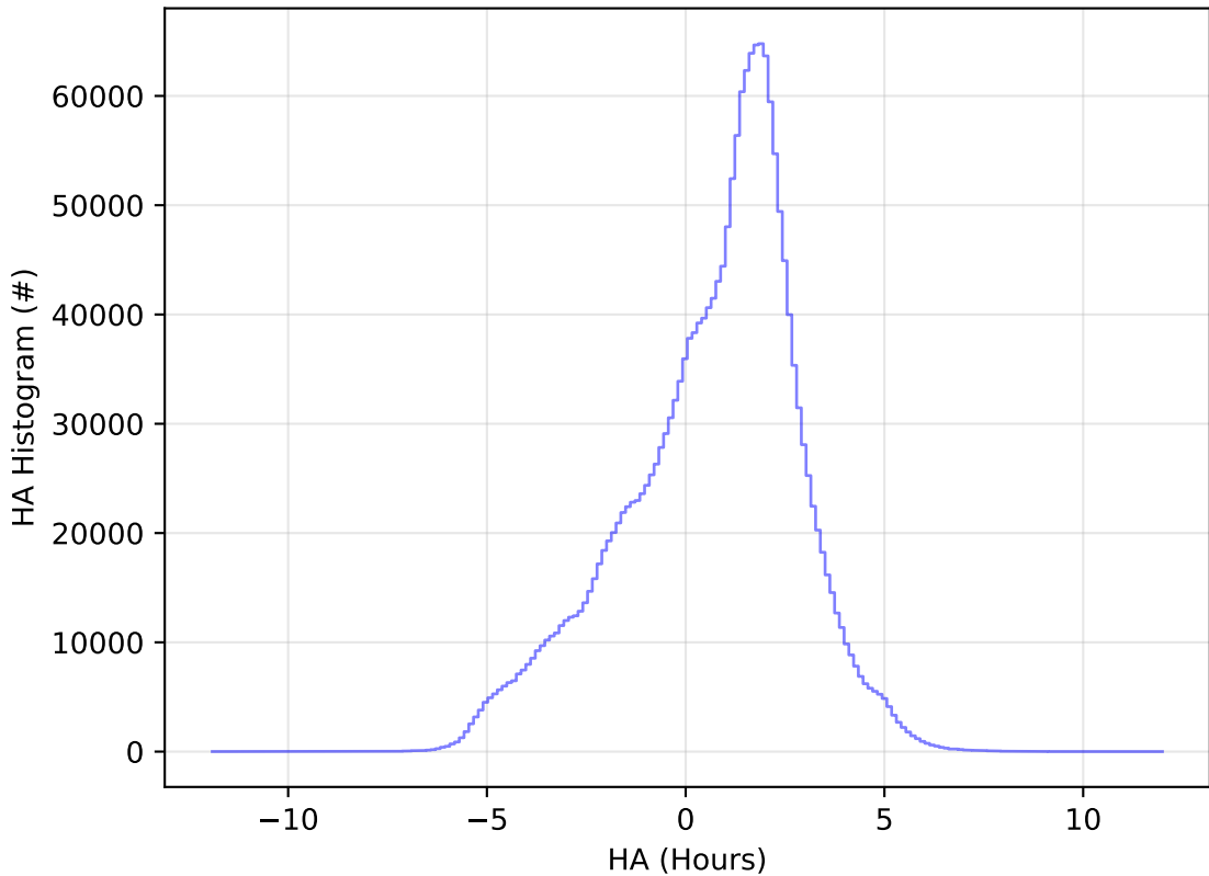
ddf_acor_sf10_lsf20_lsr50_v3.4_10yrs All sky all bands: HA Histogram
