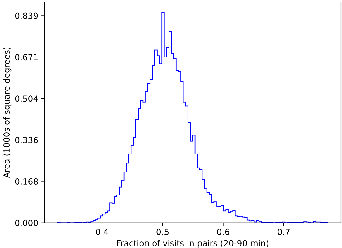
ddf_acor_sf10_lsf20_lsr50_v3.4_10yrs gri WFD: Fraction of visits in pairs (20-90 min)
