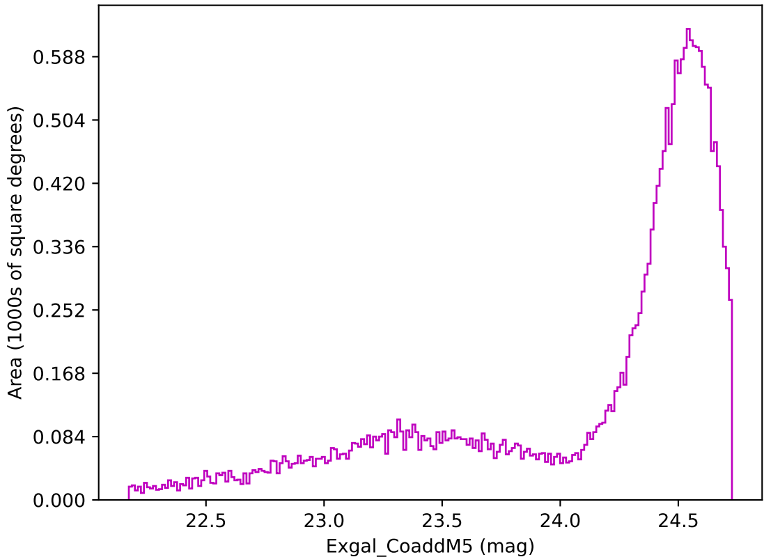
ddf_acor_sf10_lsf20_lsr50_v3.4_10yrs Yr 1 z band: Exgal_CoaddM5
