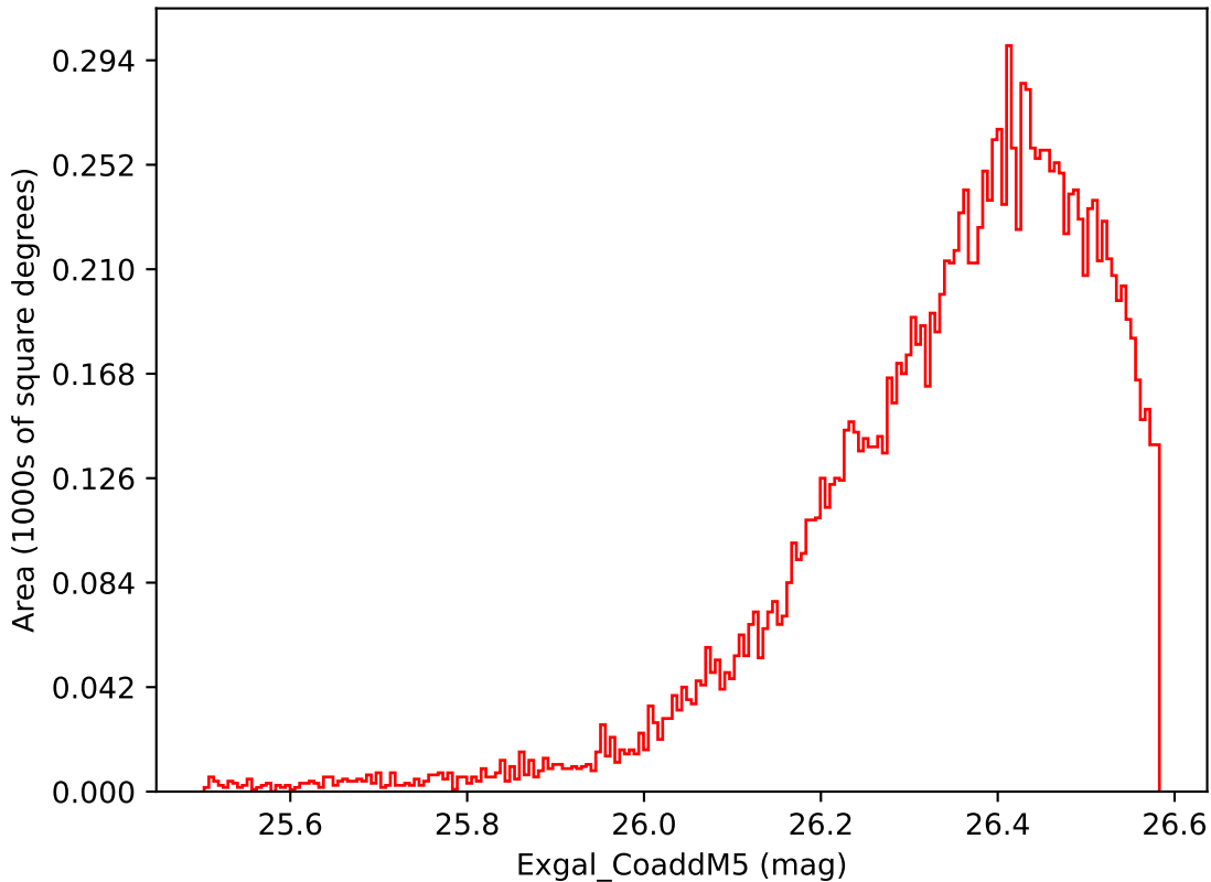
ddf_acor_sf10_lsf20_lsr50_v3.4_10yrs WFD i band: Exgal_CoaddM5
