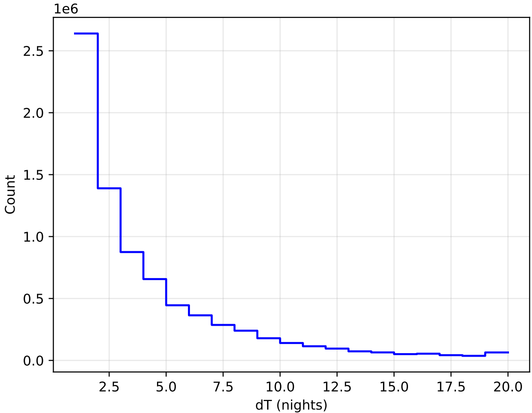
ddf_acor_sf10_lsf20_lsr50_v3.4_10yrs WFD all bands: DeltaNight Histogram
