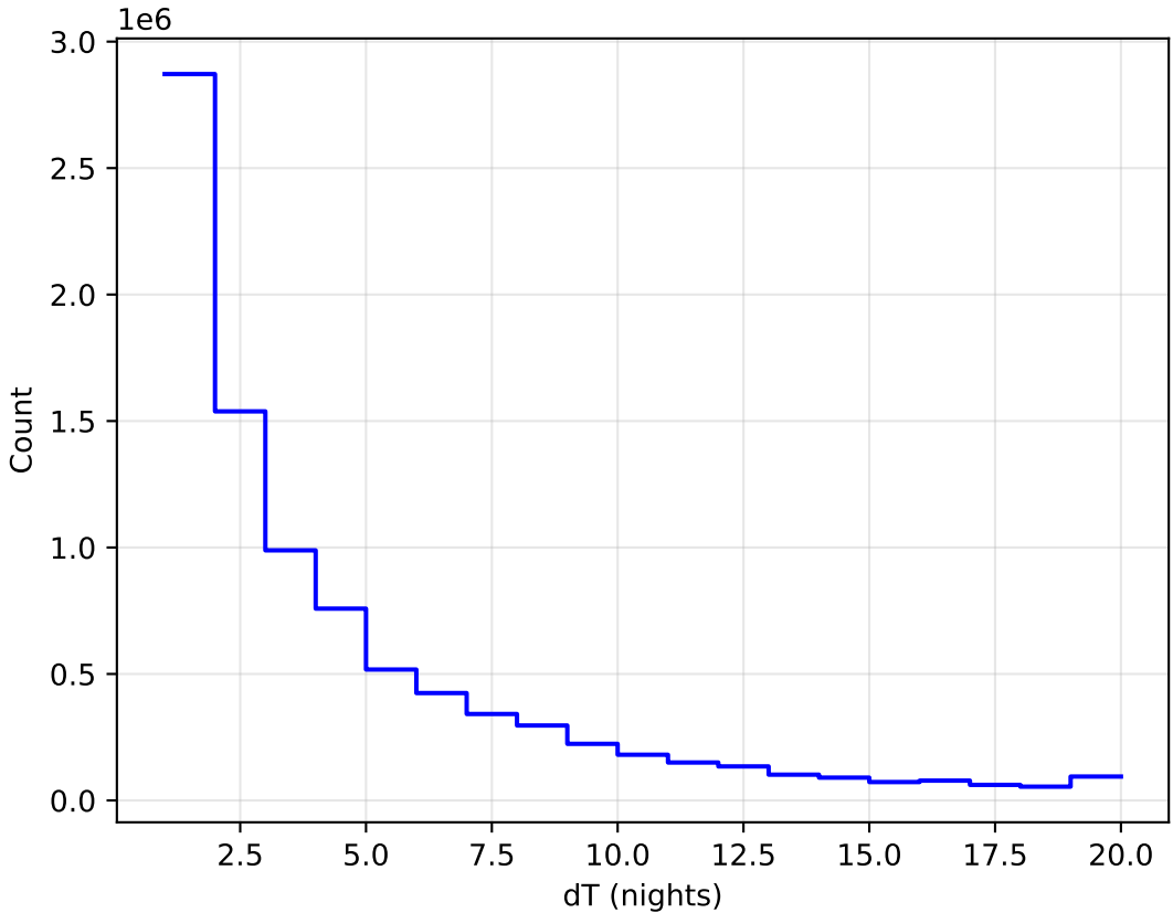
ddf_acor_sf10_lsf20_lsr50_v3.4_10yrs All sky all bands: DeltaNight Histogram
