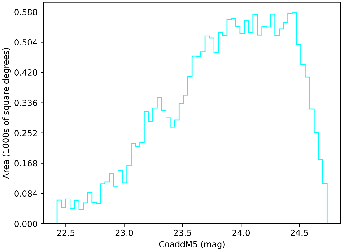
ddf_acor_sf10_lsf20_lsr50_v3.4_10yrs Yr 3-4 u band: CoaddM5
