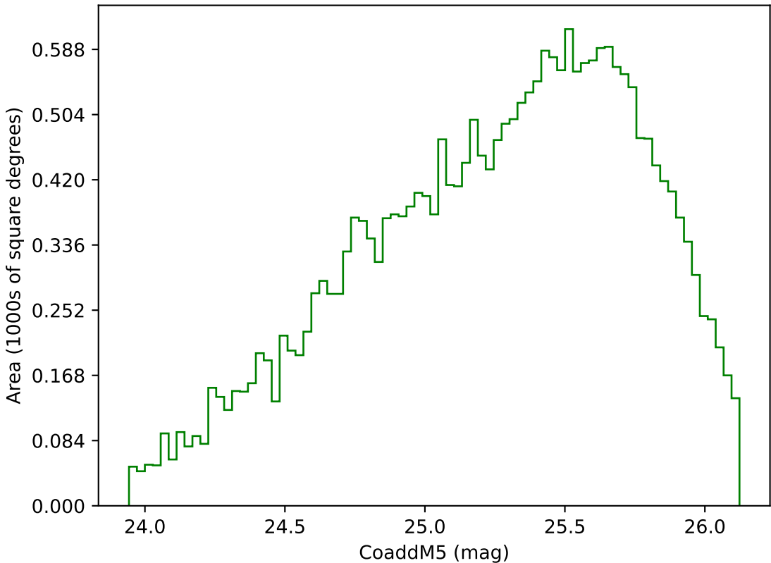
ddf_acor_sf10_lsf20_lsr50_v3.4_10yrs Yr 3-4 g band: CoaddM5
