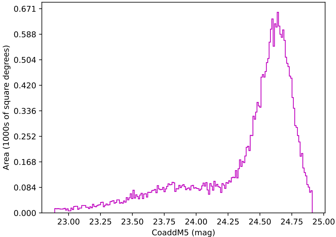
ddf_acor_sf10_lsf20_lsr50_v3.4_10yrs Yr 1 z band: CoaddM5
