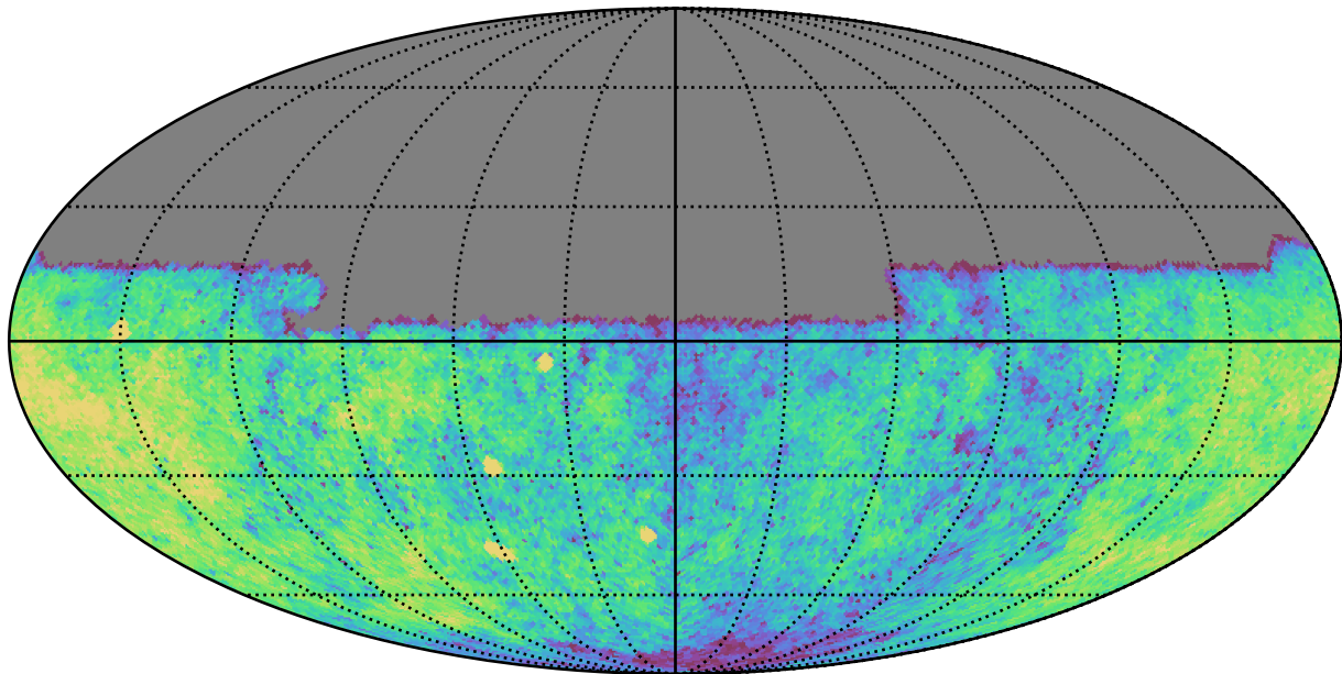
ddf_acor_sf10_lsf20_lsr50_v3.4_10yrs Yr 1 u band: CoaddM5
