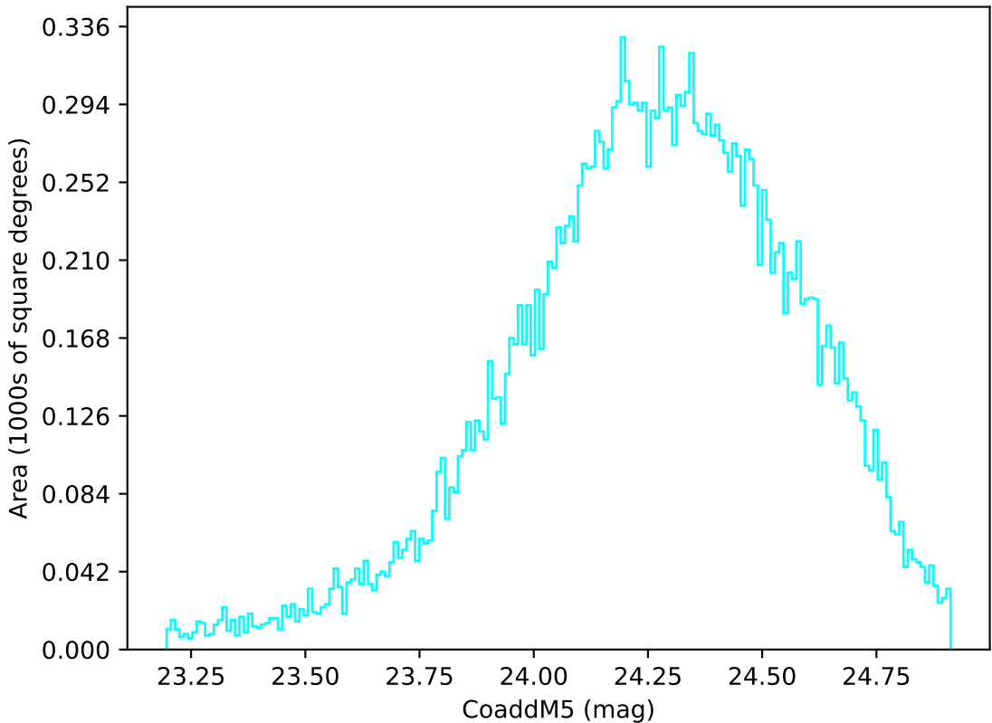
ddf_acor_sf10_lsf20_lsr50_v3.4_10yrs Yr 1 u band: CoaddM5
