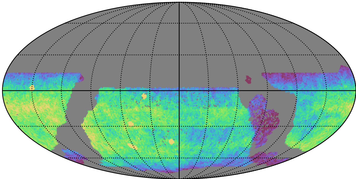
ddf_acor_sf10_lsf20_lsr50_v3.4_10yrs WFD u band: CoaddM5
