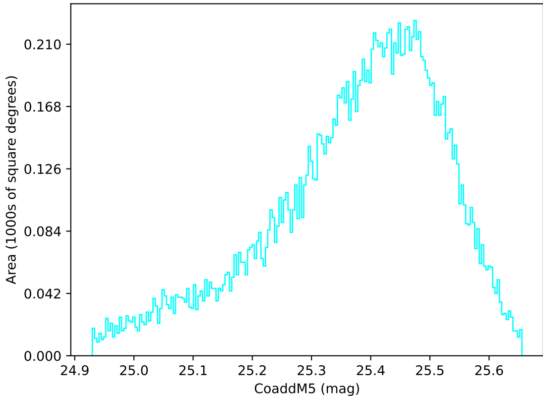
ddf_acor_sf10_lsf20_lsr50_v3.4_10yrs WFD u band: CoaddM5
