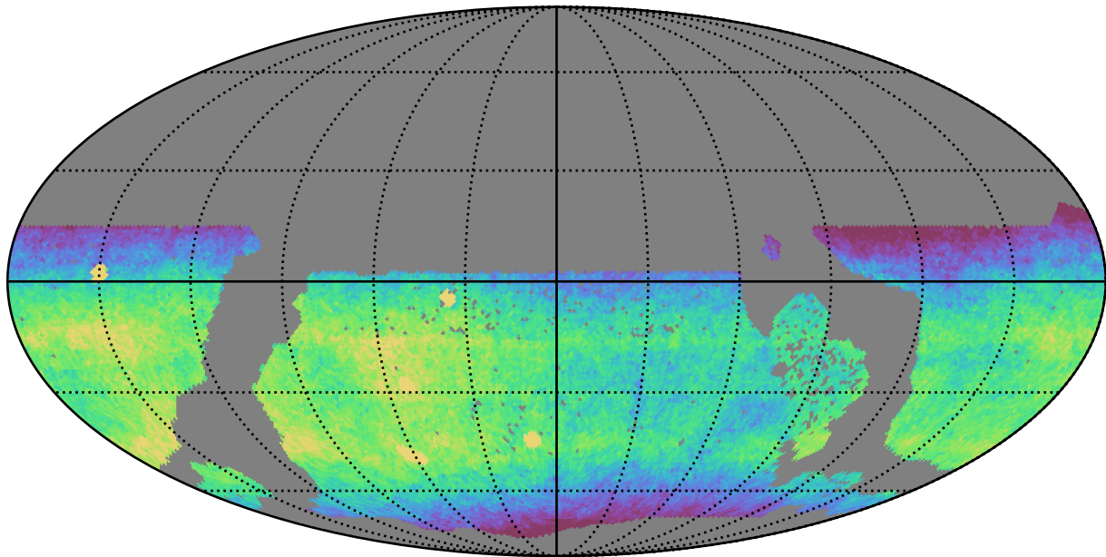
ddf_acor_sf10_lsf20_lsr50_v3.4_10yrs WFD i band: CoaddM5
