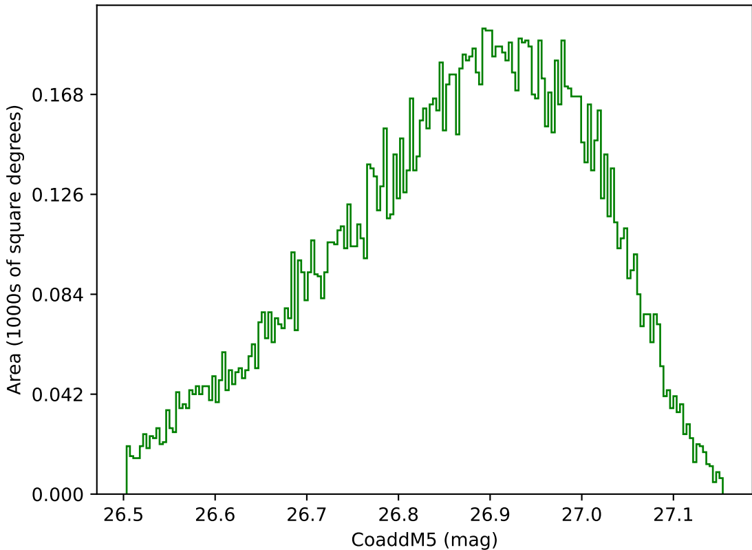
ddf_acor_sf10_lsf20_lsr50_v3.4_10yrs WFD g band: CoaddM5
