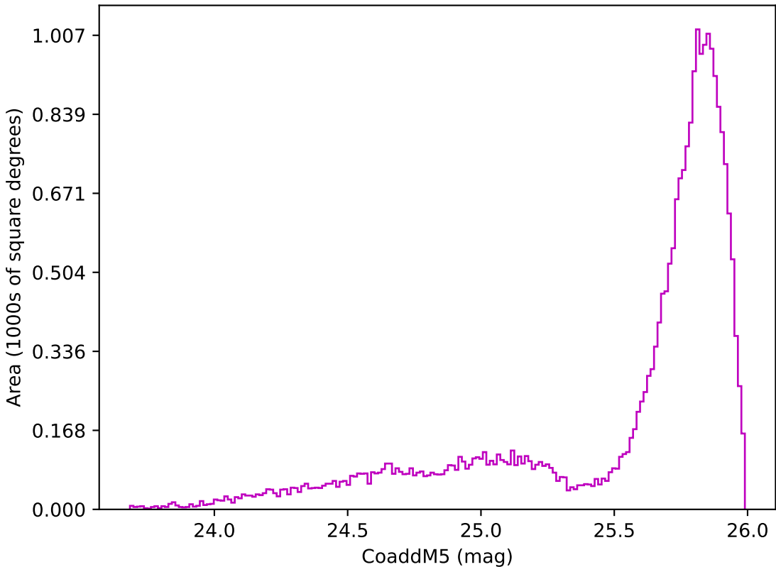
ddf_acor_sf10_lsf20_lsr50_v3.4_10yrs All sky z band: CoaddM5
