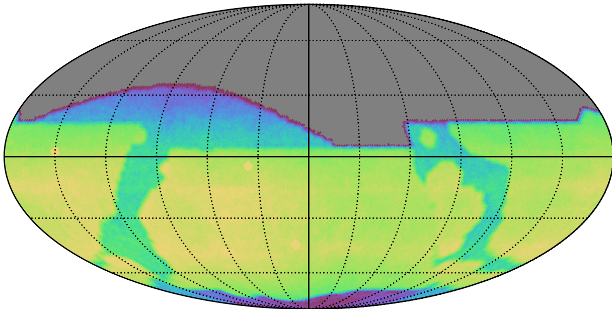
ddf_acor_sf10_lsf20_lsr50_v3.4_10yrs All sky r band: CoaddM5
