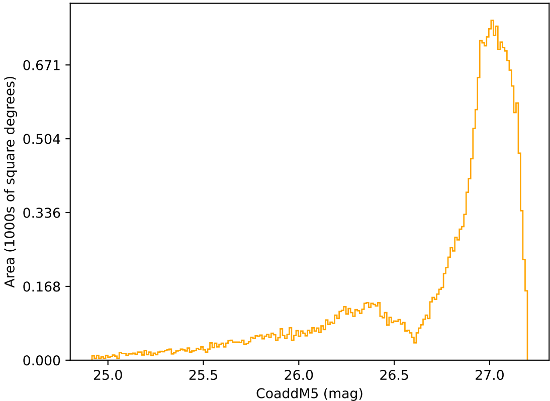
ddf_acor_sf10_lsf20_lsr50_v3.4_10yrs All sky r band: CoaddM5
