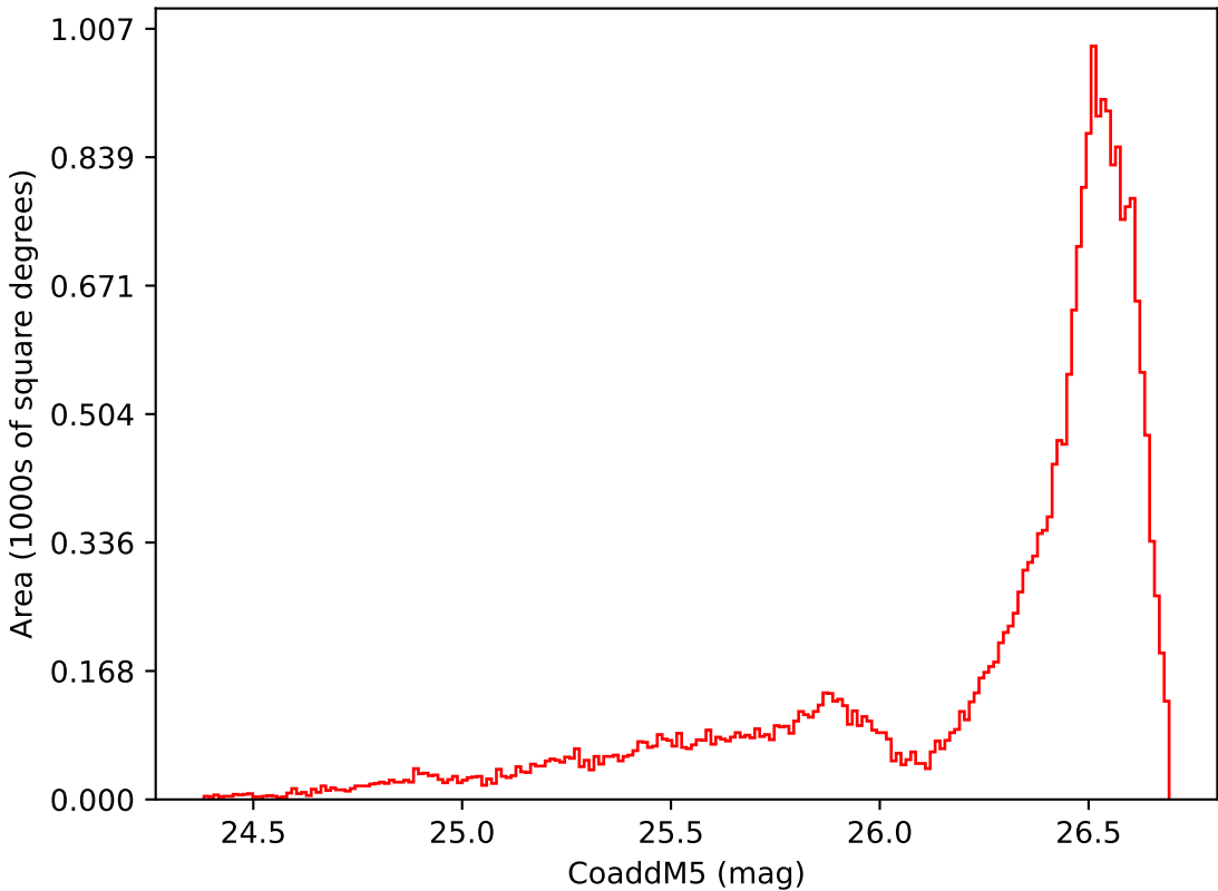
ddf_acor_sf10_lsf20_lsr50_v3.4_10yrs All sky i band: CoaddM5
