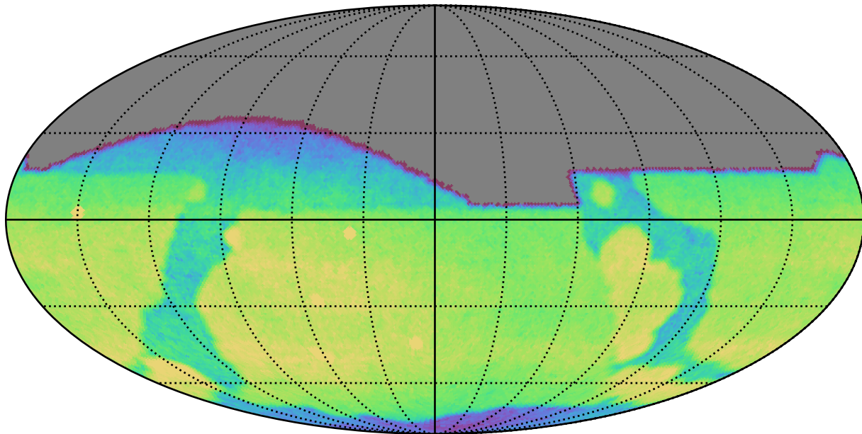
ddf_acor_sf10_lsf20_lsr50_v3.4_10yrs All sky g band: CoaddM5
