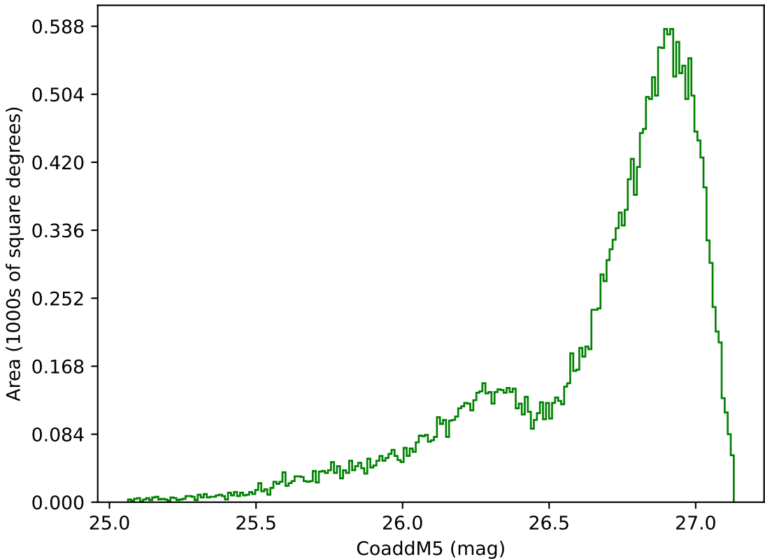
ddf_acor_sf10_lsf20_lsr50_v3.4_10yrs All sky g band: CoaddM5
