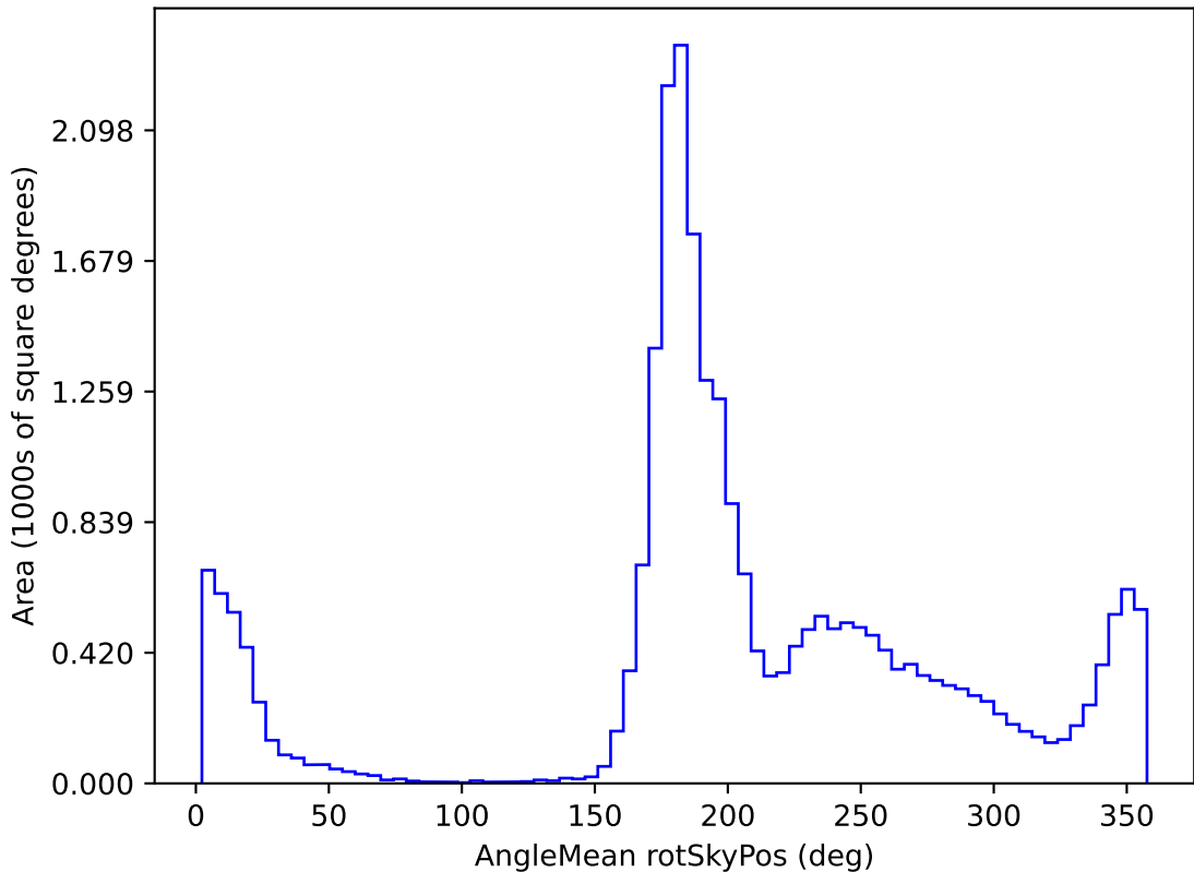
ddf_acor_sf10_lsf20_lsr50_v3.4_10yrs All sky i band: AngleMean rotSkyPos
