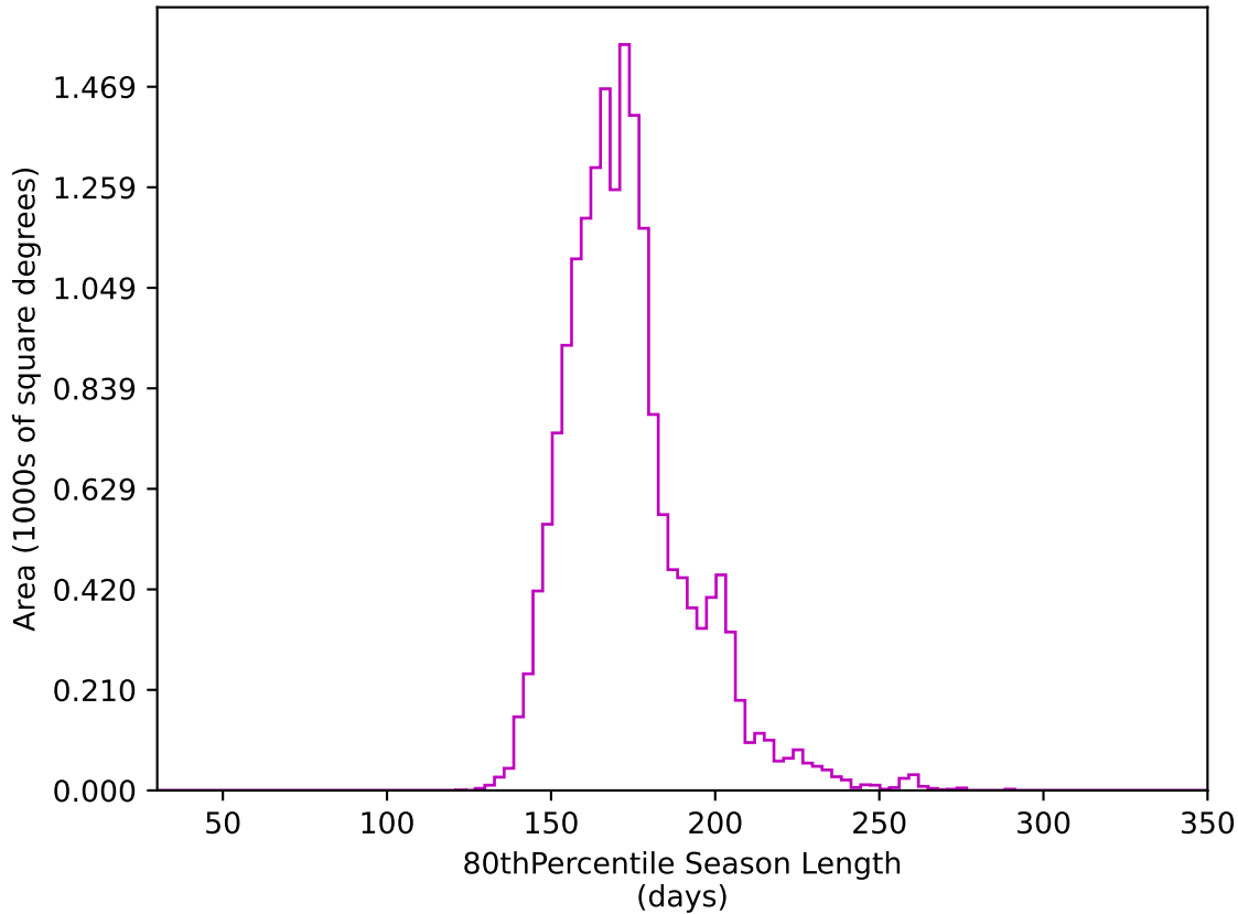
ddf_acor_sf10_lsf20_lsr50_v3.4_10yrs WFD z band: 80thPercentile Season Length
