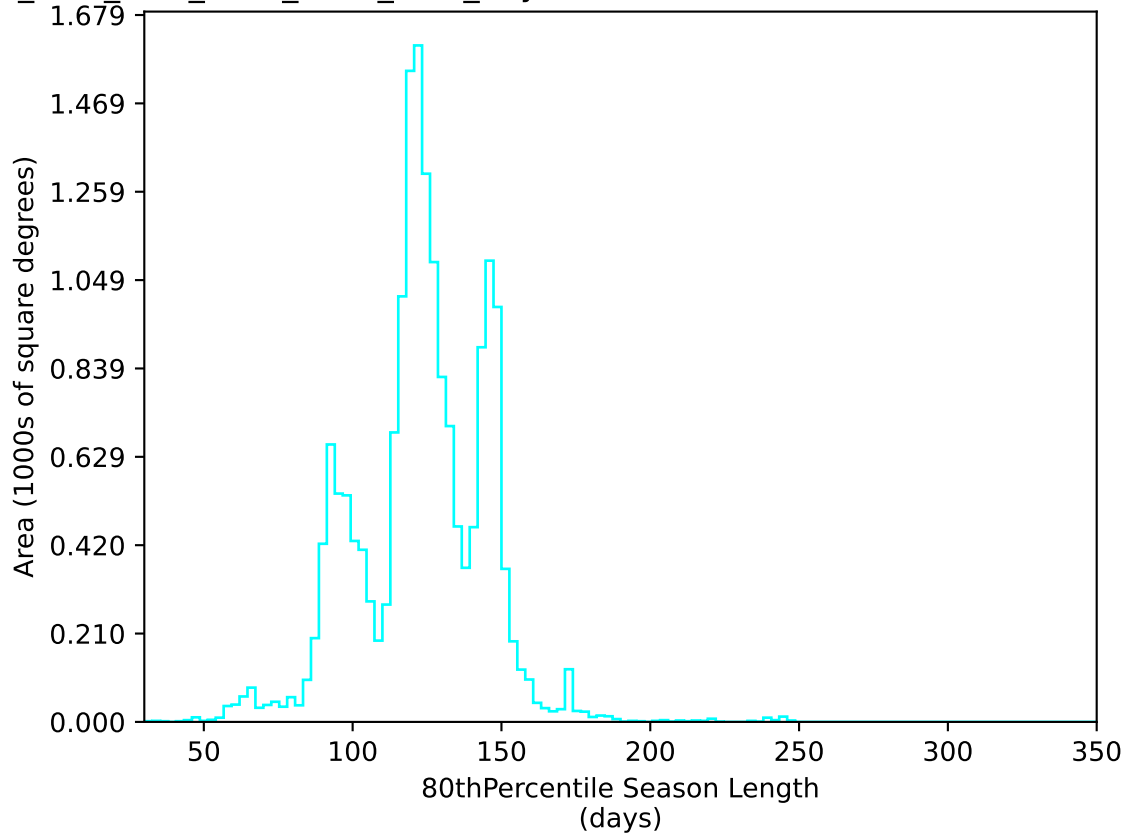
ddf_acor_sf10_lsf20_lsr50_v3.4_10yrs WFD u band: 80thPercentile Season Length
