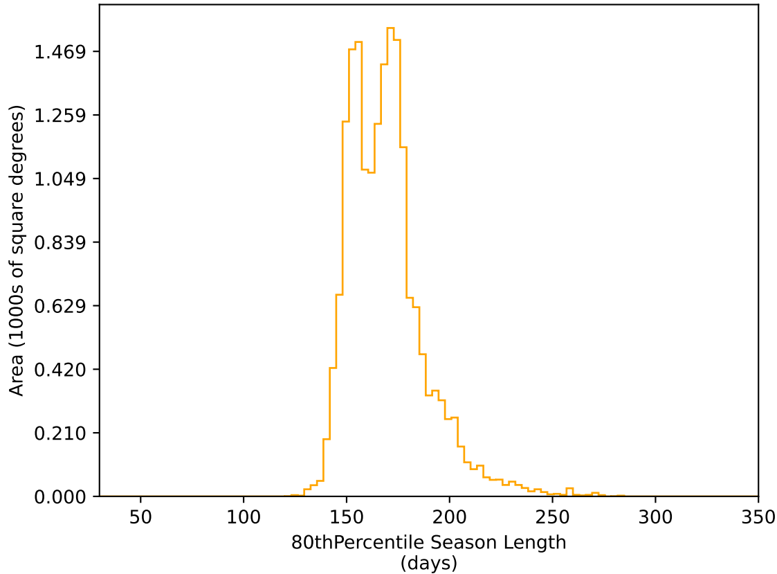
ddf_acor_sf10_lsf20_lsr50_v3.4_10yrs WFD r band: 80thPercentile Season Length
