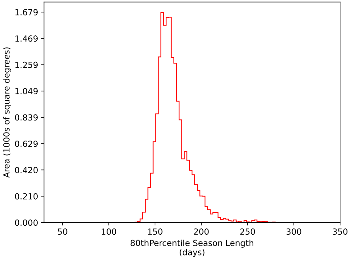
ddf_acor_sf10_lsf20_lsr50_v3.4_10yrs WFD i band: 80thPercentile Season Length
