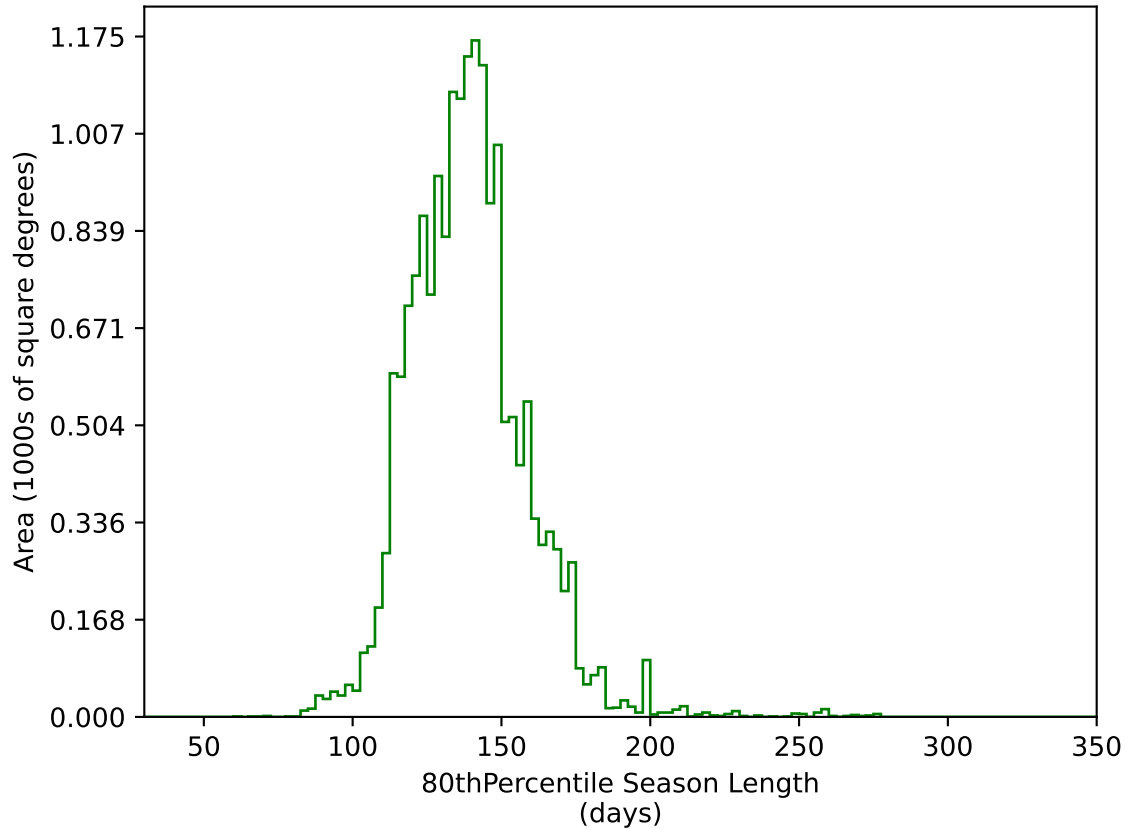
ddf_acor_sf10_lsf20_lsr50_v3.4_10yrs WFD g band: 80thPercentile Season Length
