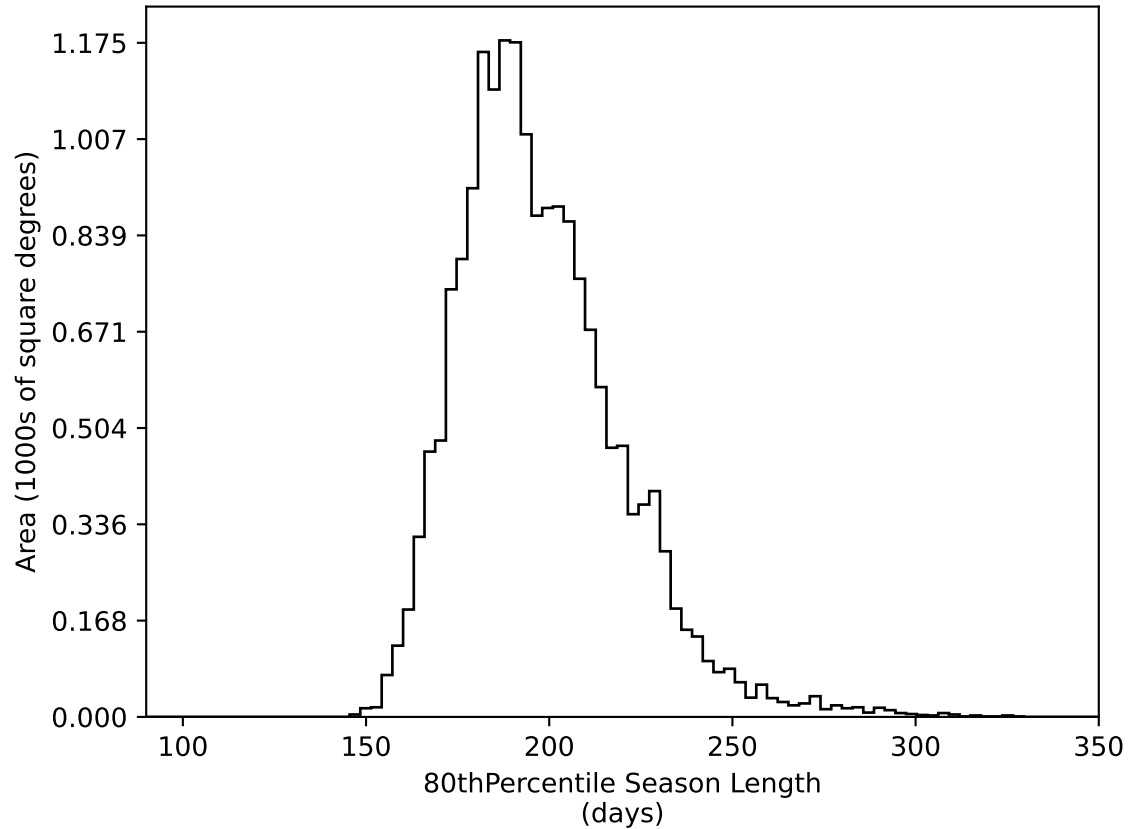
ddf_acor_sf10_lsf20_lsr50_v3.4_10yrs WFD all bands: 80thPercentile Season Length
