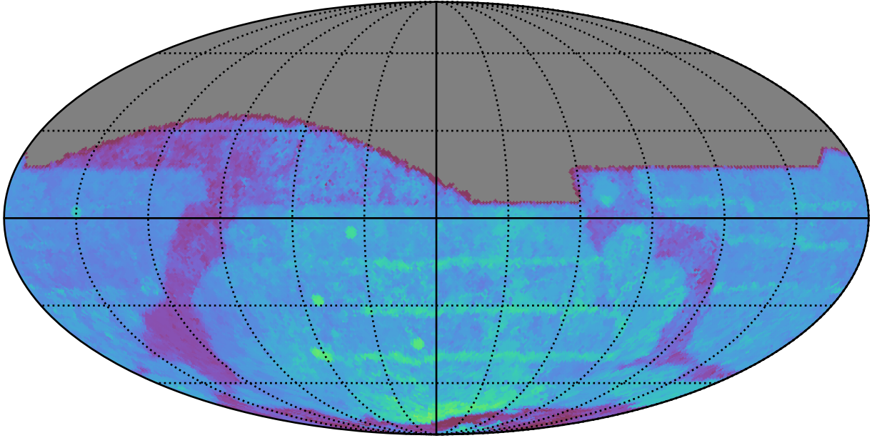
ddf_acor_sf10_lsf20_lsr50_v3.4_10yrs All sky z band: 80thPercentile Season Length
