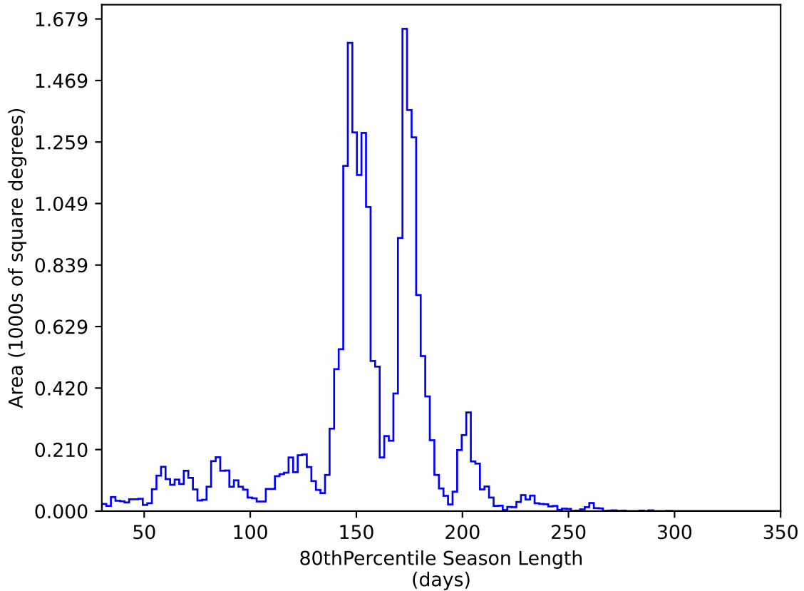
ddf_acor_sf10_lsf20_lsr50_v3.4_10yrs All sky y band: 80thPercentile Season Length
