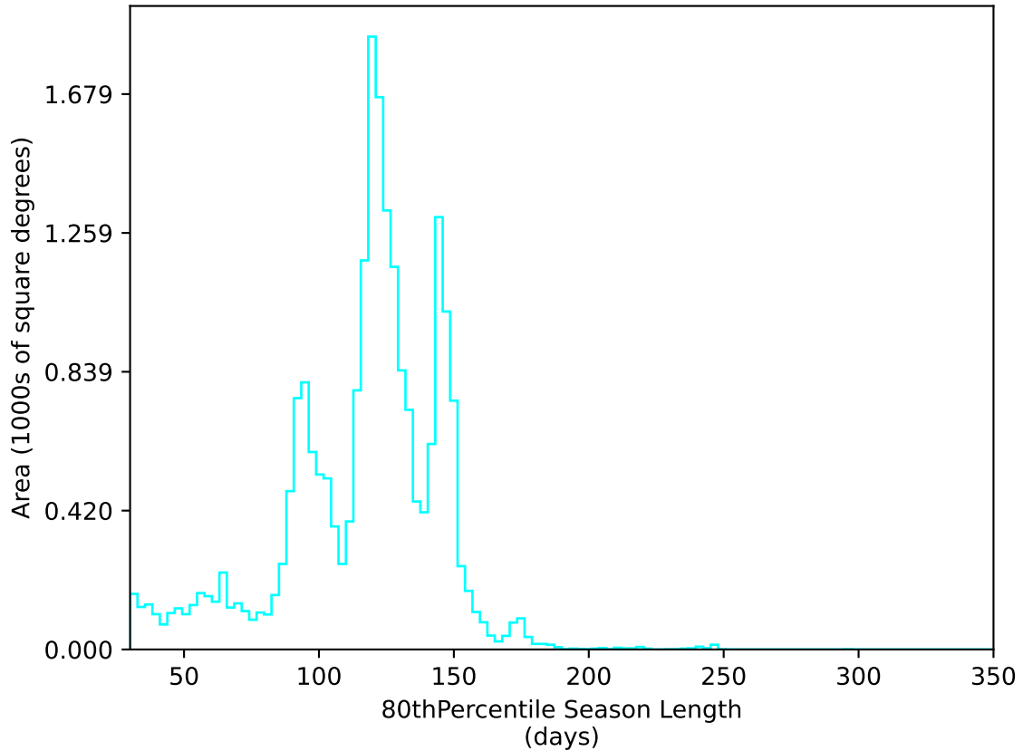
ddf_acor_sf10_lsf20_lsr50_v3.4_10yrs All sky u band: 80thPercentile Season Length
