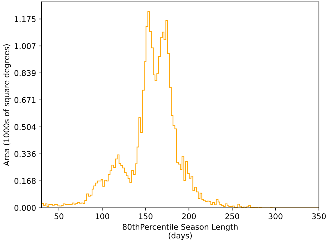
ddf_acor_sf10_lsf20_lsr50_v3.4_10yrs All sky r band: 80thPercentile Season Length
