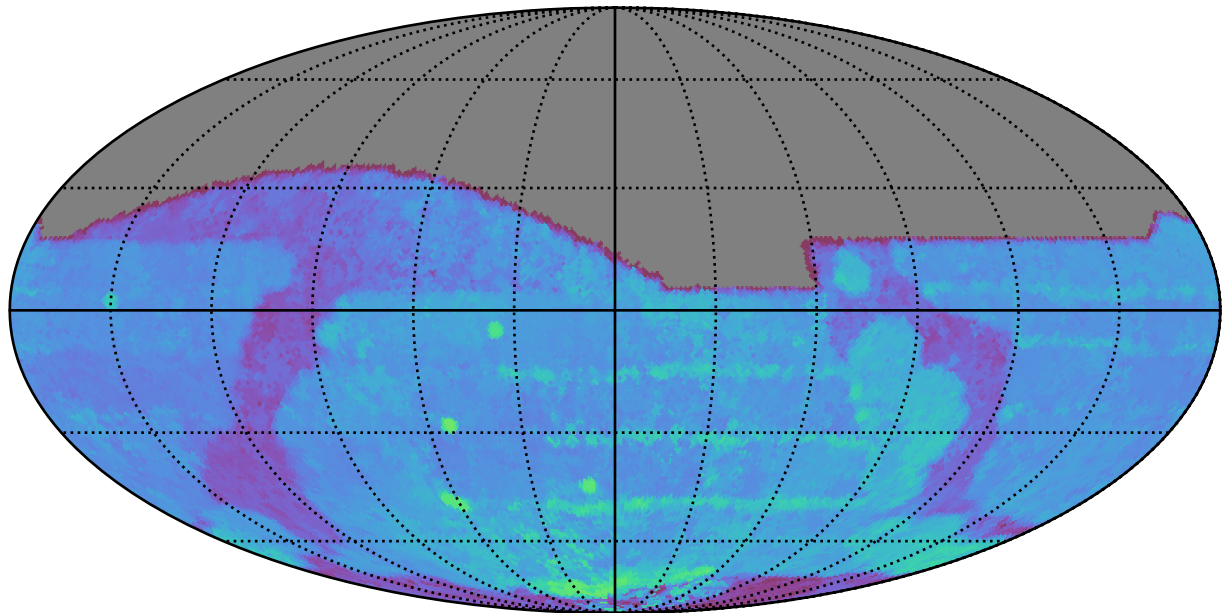
ddf_acor_sf10_lsf20_lsr50_v3.4_10yrs All sky i band: 80thPercentile Season Length
