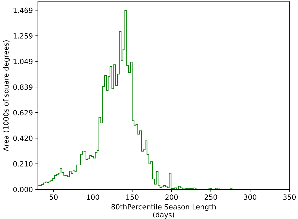
ddf_acor_sf10_lsf20_lsr50_v3.4_10yrs All sky g band: 80thPercentile Season Length
