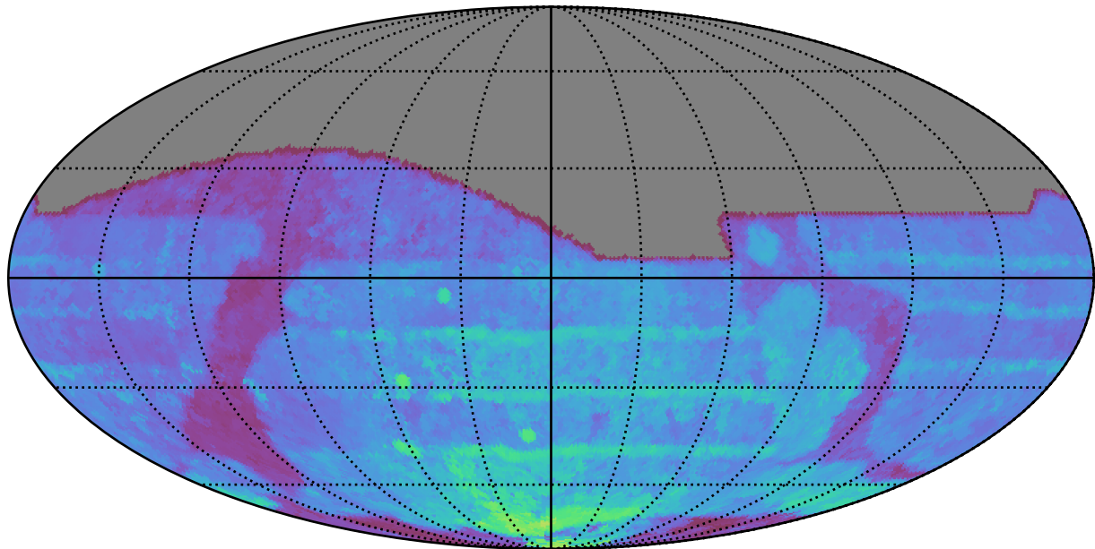
ddf_acor_sf10_lsf20_lsr50_v3.4_10yrs All sky all bands: 80thPercentile Season Length
