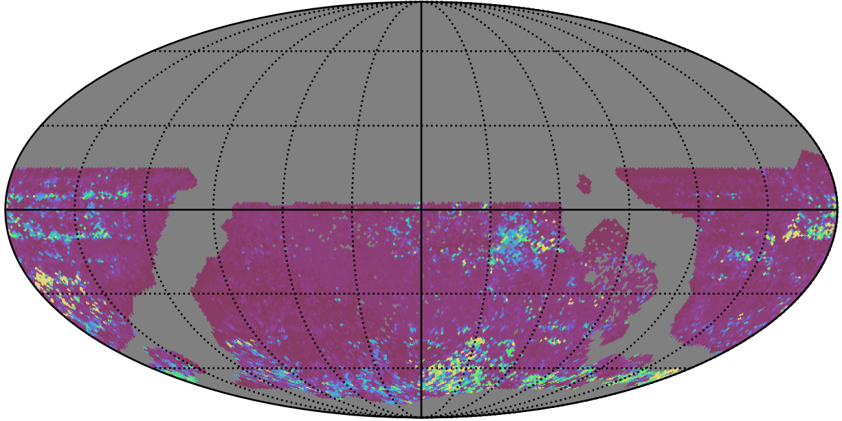
ddf_acor_sf10_lsf20_lsr50_v3.4_10yrs WFD z band: 75th Percentile Intranight Timespan
