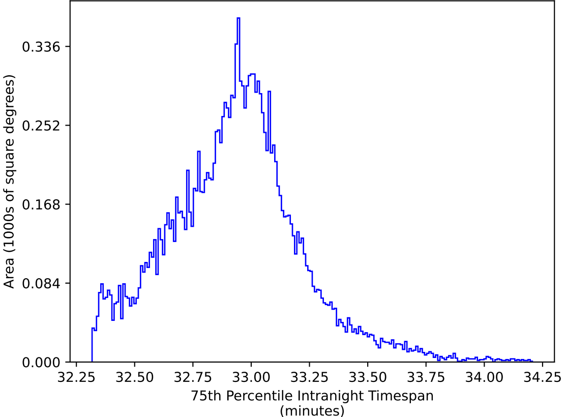
ddf_acor_sf10_lsf20_lsr50_v3.4_10yrs WFD y band: 75th Percentile Intranight Timespan
