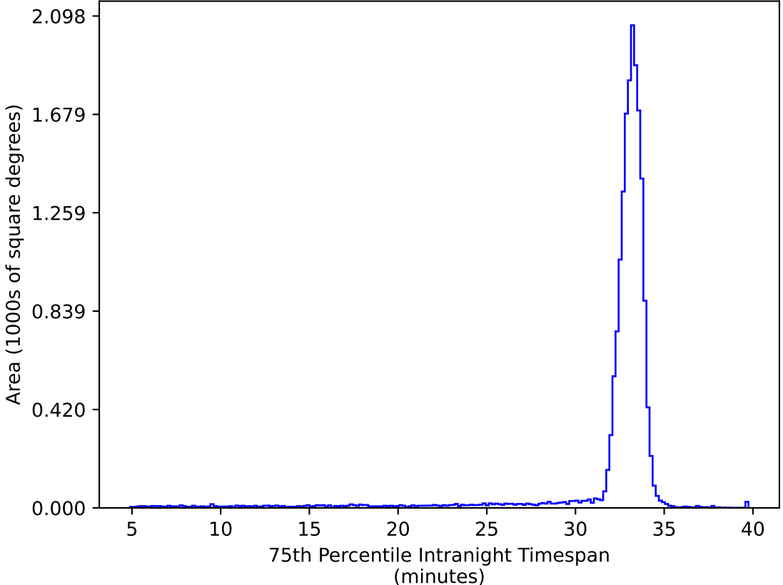
ddf_acor_sf10_lsf20_lsr50_v3.4_10yrs WFD ug bands: 75th Percentile Intranight Timespan
