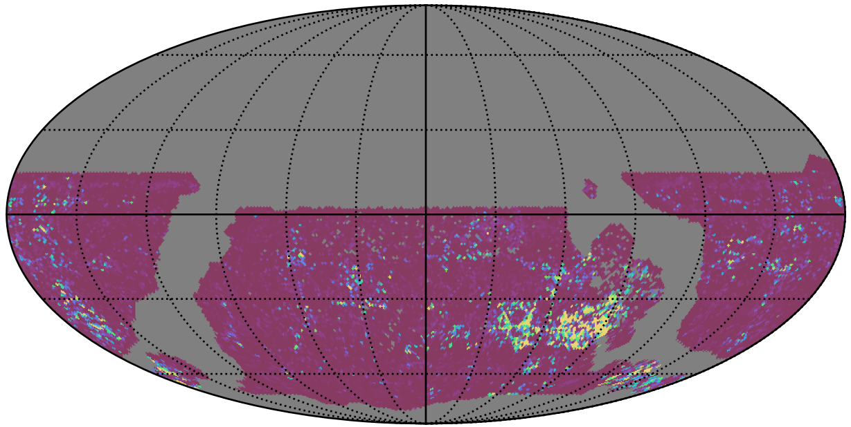
ddf_acor_sf10_lsf20_lsr50_v3.4_10yrs WFD u band: 75th Percentile Intranight Timespan
