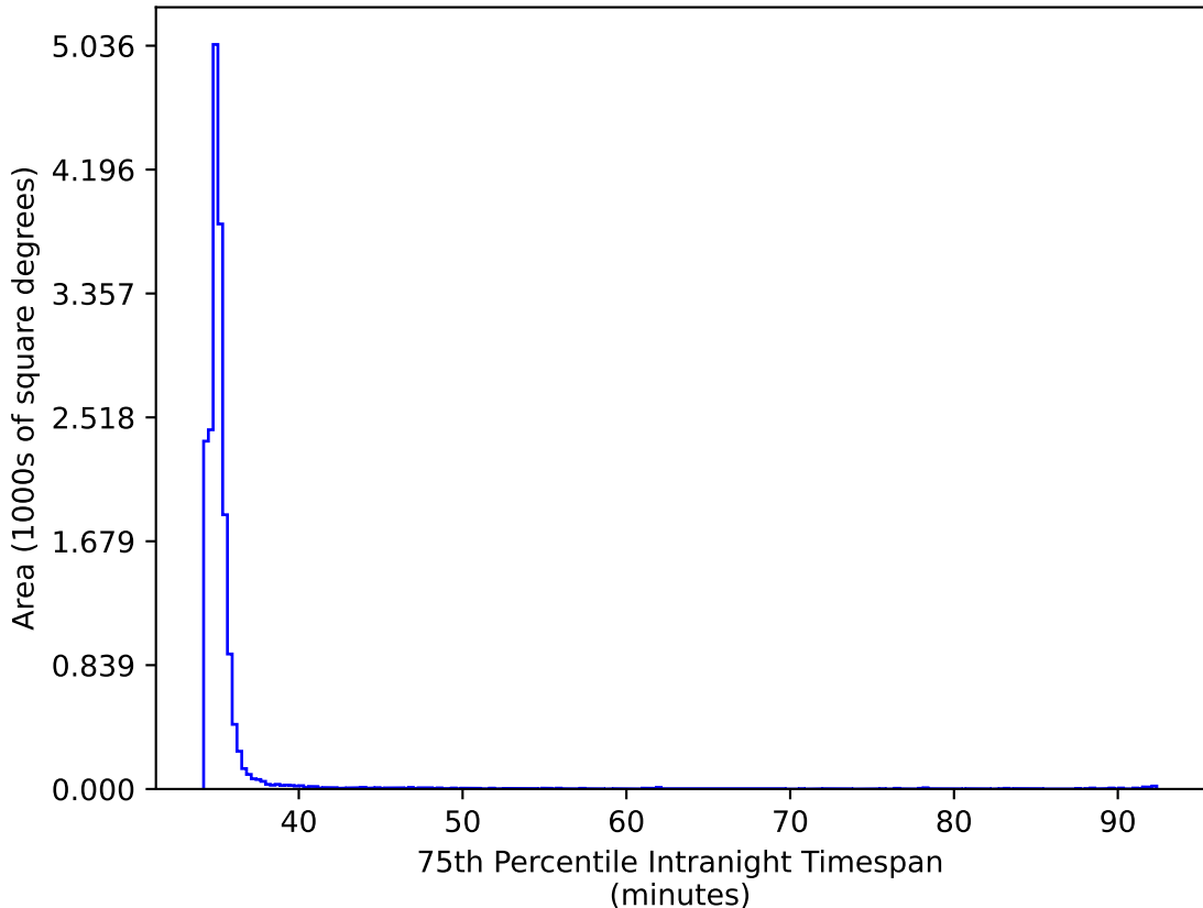
ddf_acor_sf10_lsf20_lsr50_v3.4_10yrs WFD ri bands: 75th Percentile Intranight Timespan
