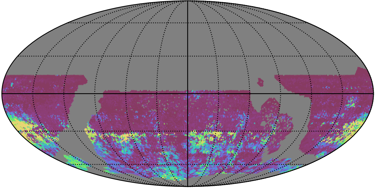
ddf_acor_sf10_lsf20_lsr50_v3.4_10yrs WFD r band: 75th Percentile Intranight Timespan
