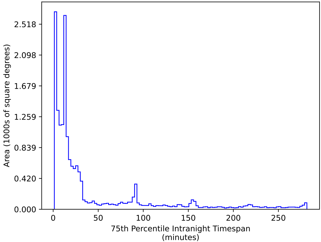
ddf_acor_sf10_ls20_lsr50_v3.4_10yrs WFD r band: 75th Percentile Intranight Timespan
