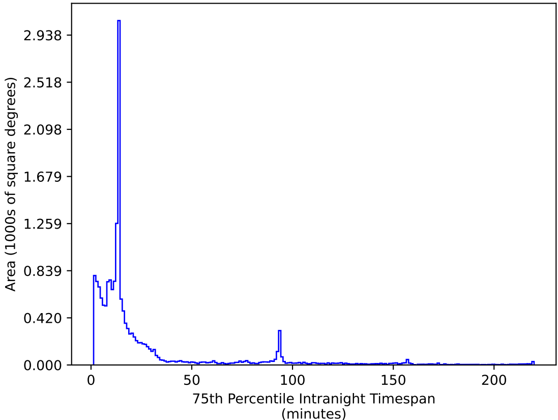
ddf_acor_sf10_lsf20_lsr50_v3.4_10yrs WFD i band: 75th Percentile Intranight Timespan
