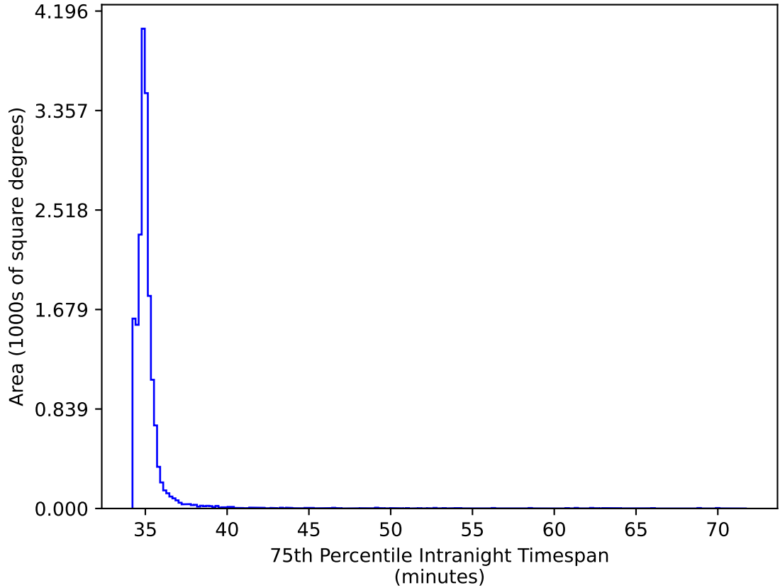
ddf_acor_sf10_lsf20_lsr50_v3.4_10yrs WFD gr bands: 75th Percentile Intranight Timespan
