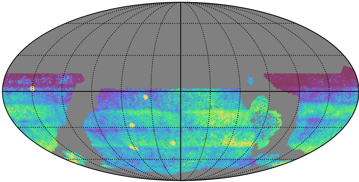
ddf_acor_sf10_lsf20_lsr50_v3.4_10yrs WFD all bands: 75th Percentile Intranight Timespan
