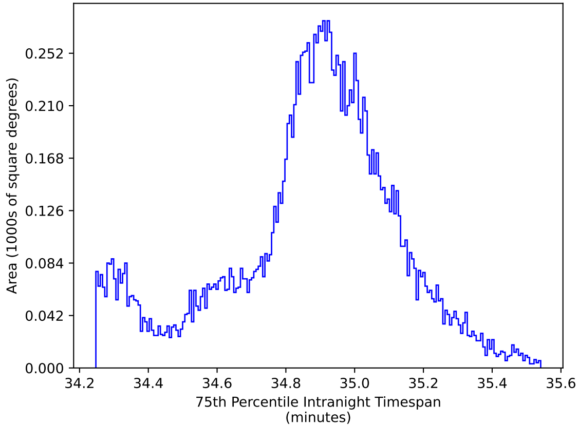
ddf_acor_sf10_lsf20_lsr50_v3.4_10yrs WFD all bands: 75th Percentile Intranight Timespan
