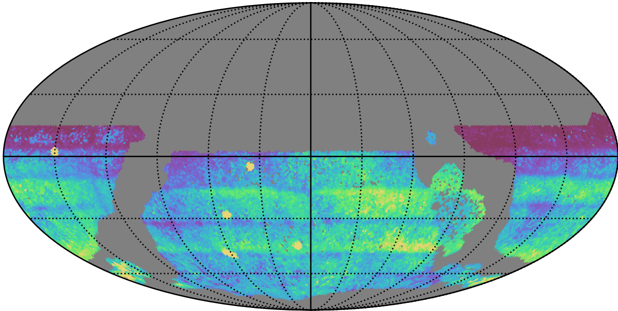
ddf_acor_sf10_lsf20_lsr50_v3.4_10yrs WFD: 75th Percentile Intranight Timespan
